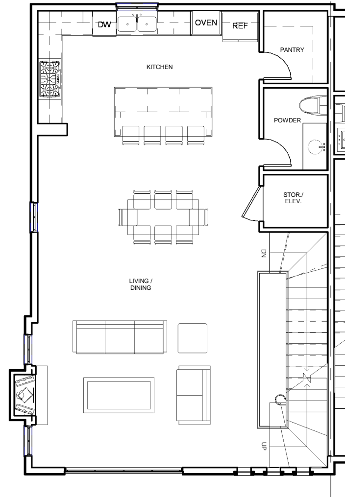
SECOND FLOOR PLAN UNIT 'A' SCALE: 1/8" = 1'-0"
