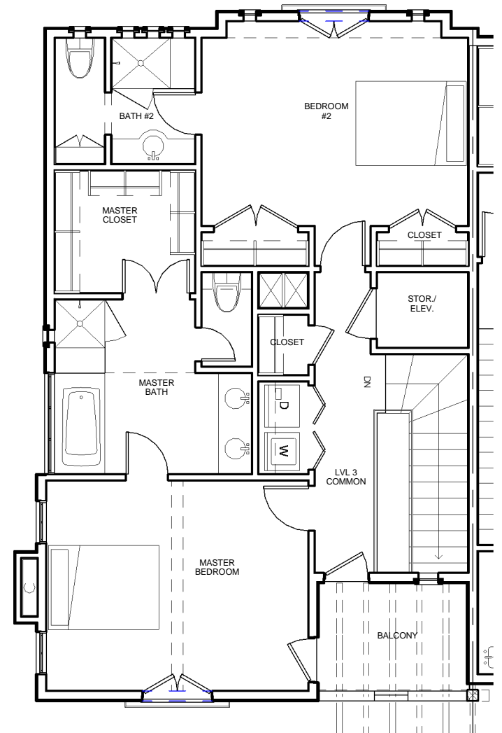
THIRD FLOOR PLAN UNIT 'A' SCALE: 1/8" = 1'-0"
