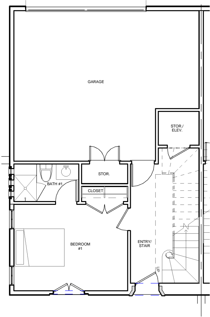
FIRST FLOOR PLAN UNIT 'A' SCALE: 1/8" = 1'-0"
